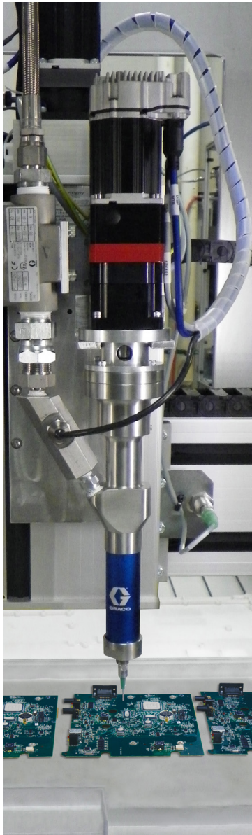
The Graco PC pump in use at a major electronics supplier
